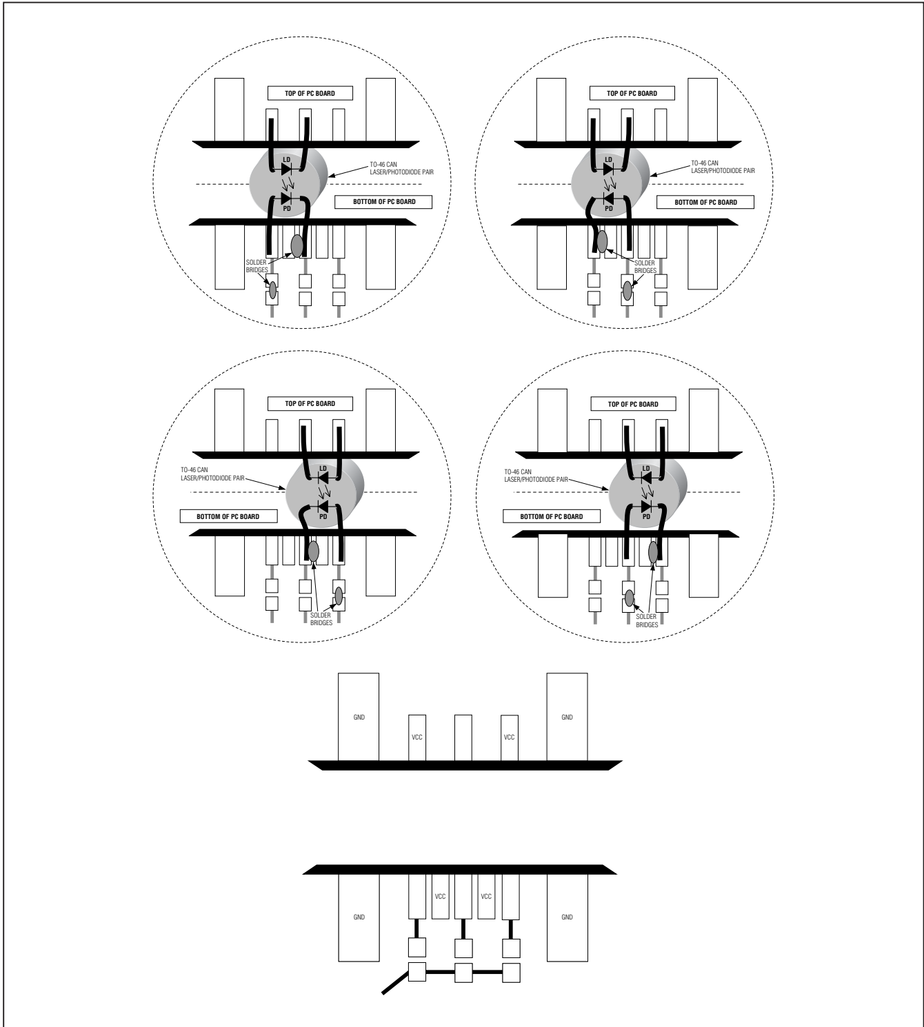
Figure 1. Laser Diode/Monitor Diode Attachment to the MAX3863 EV Kit
