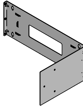
ITEM 3 HINGED BRACKET QTY 1
