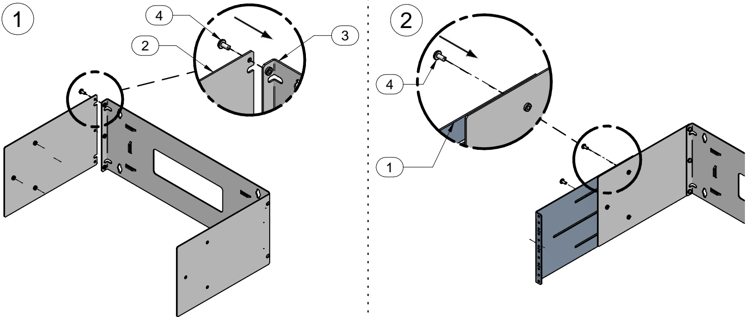
ITEM 1 TAPPED SLIDE RAIL QTY 2
