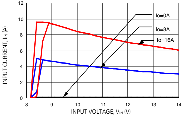
Figure 7. Input voltage vs. Input Current (V out = 5.0Vdc).
