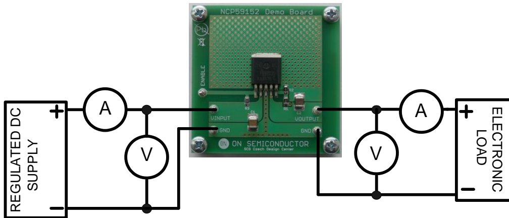
Figure 1: Test Setup
