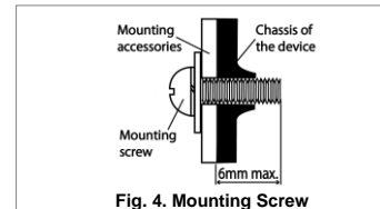
Fig. 4. Mounting Screw
