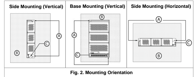
Fig. 2. Mounting Orientation
