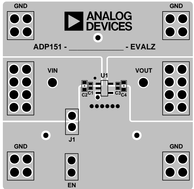
Figure 4. ADP151UJZ-RedyKit Evaluation Board Layout
