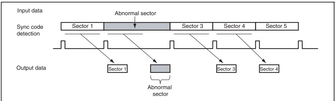
Figure 23.11 Operation in External Sync Mode
