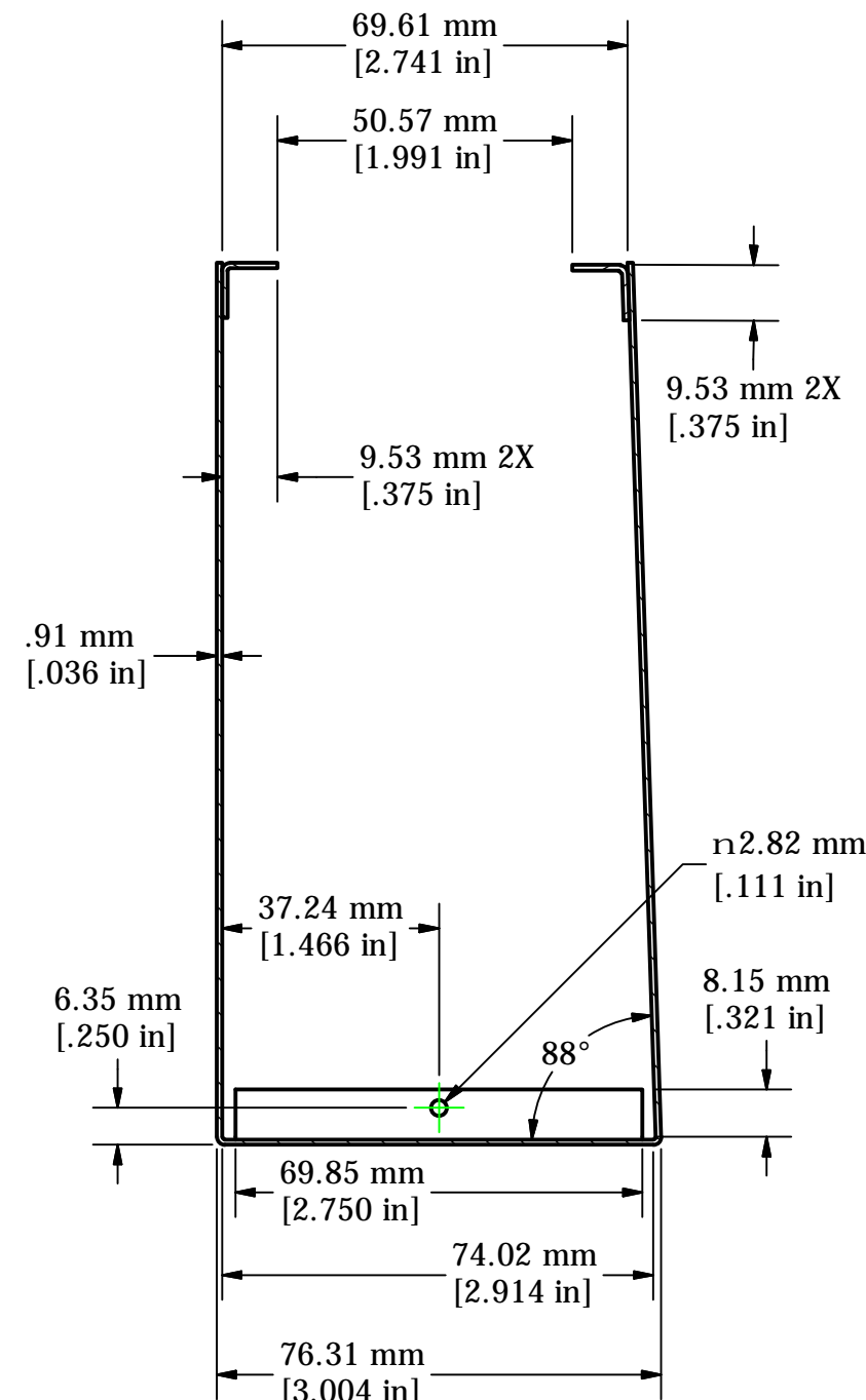
SECTION A-A SIDE SECTION VIEW OF EXPLODED ASSEMBLY
