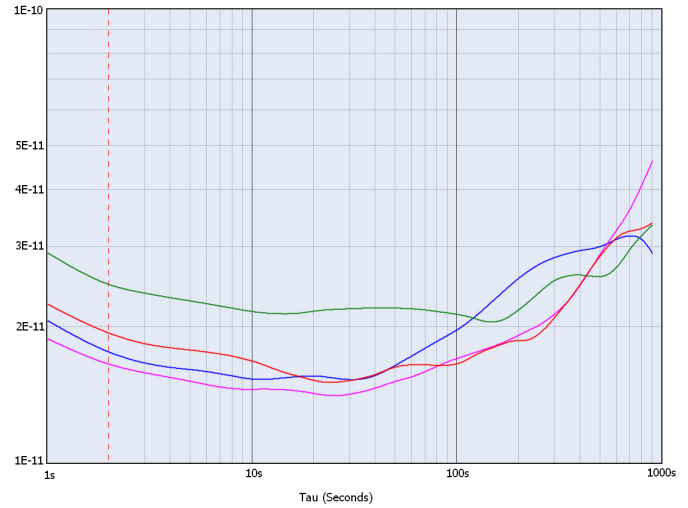
Allan Deviation DOCSC012F-024.576M
