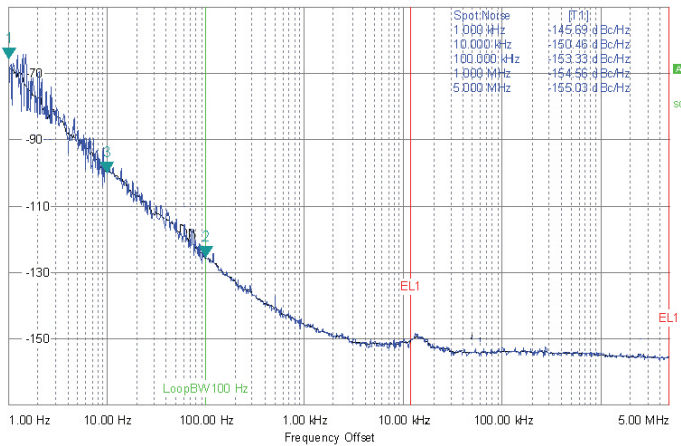
Typical Phase Noise for DOCSC012F-024.57M
