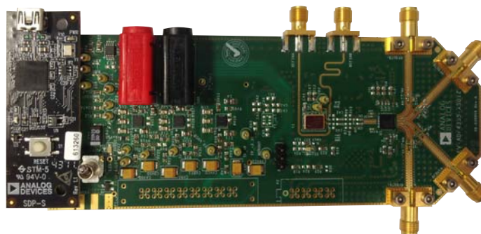
Figure 1. EV-ADF4355-2SD1Z
